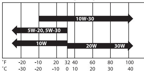
TEMPERATURE CHART
